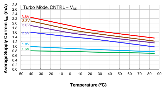
Average Supply Current (CNTRL = V_{DD} ) vs Temperature
