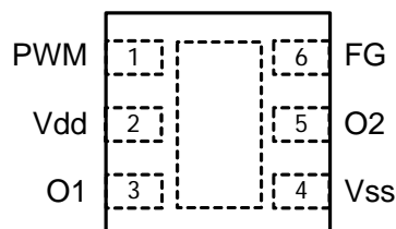
DFN2020C-6
