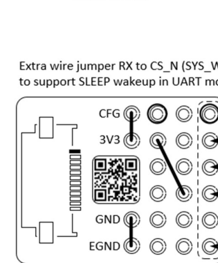
Wire jumper to short EGND to GND
