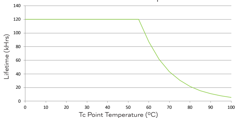
Lifetime Vs. Tcase Temp
