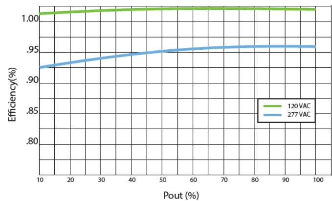
Power Factor vs. Output Power - 0-10V-Dimming
