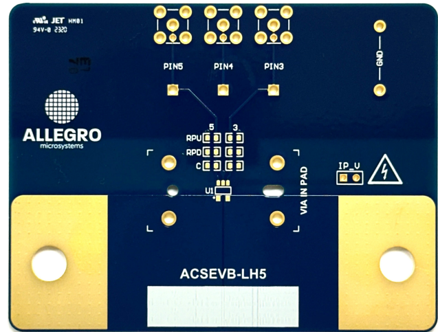
Figure 1: LH Bare Evaluation Board
