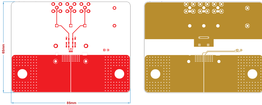
Figure 8: LH Generic Evaluation Board Top Layer (left) and Interior Layer 1
