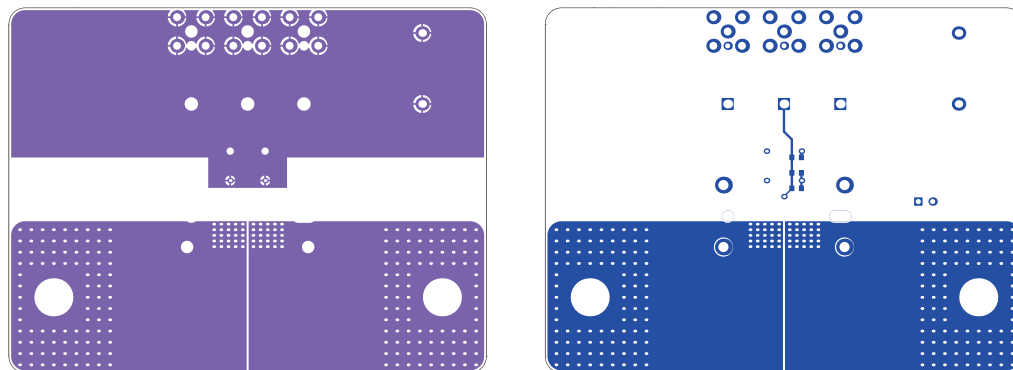
Figure 10: LH Generic Evaluation Board Interior Layer 4 (left) and Bottom Layer
