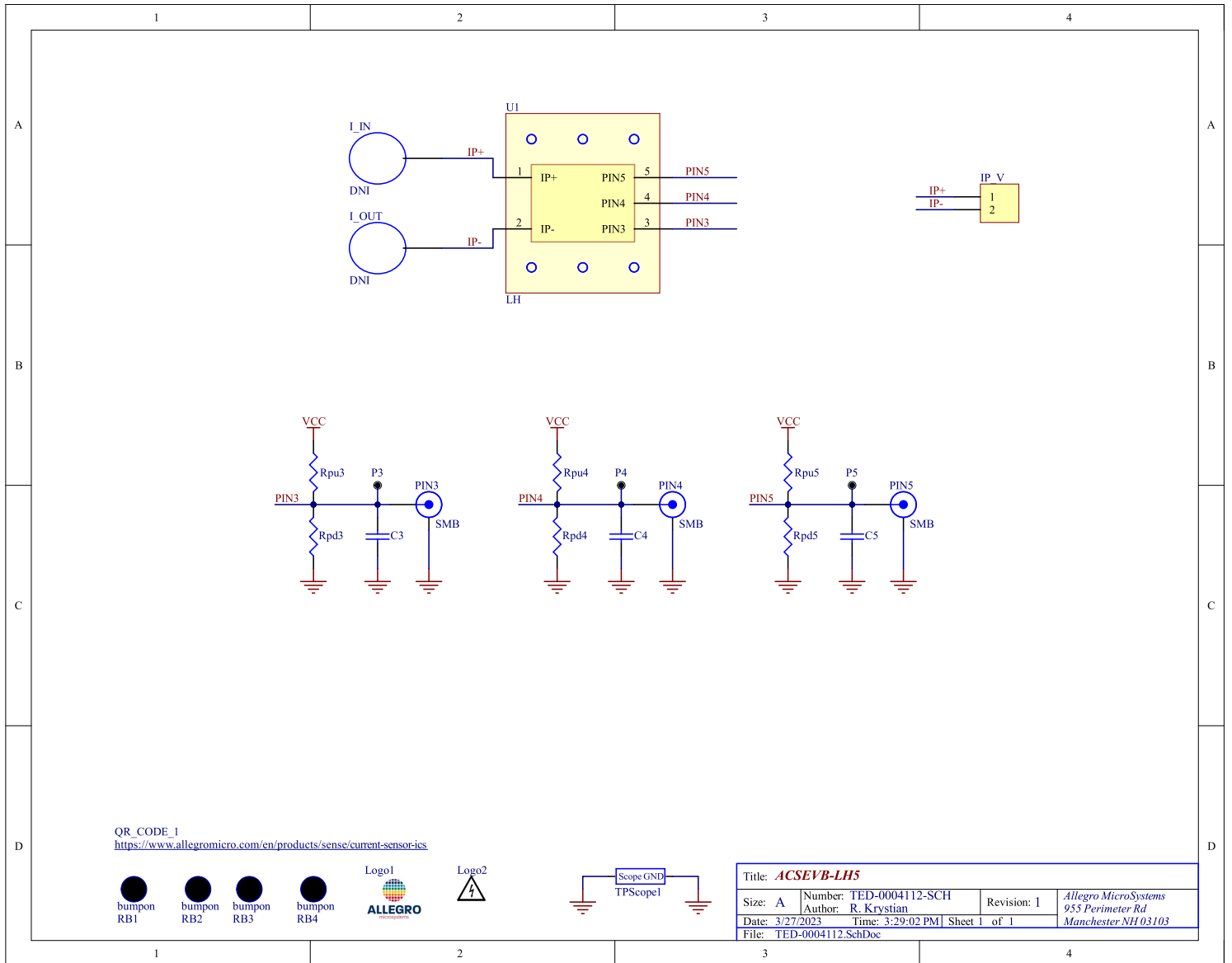
Figure 7: LH Generic Evaluation Board Schematic
