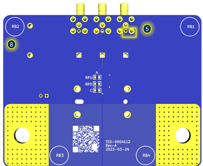
Bottom view
