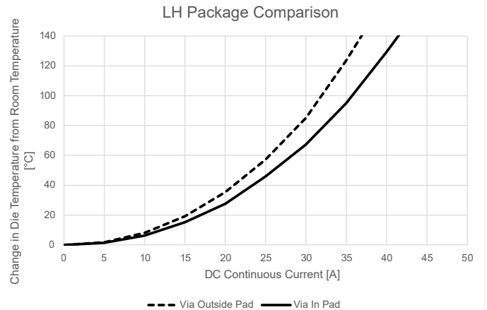
Figure 6: LH Package Comparison with and without In-Pad Vias
