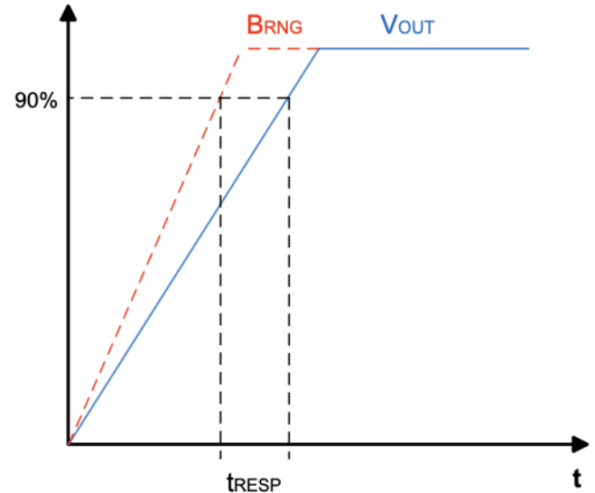
Figure 22. CT453 Response Time Curve
