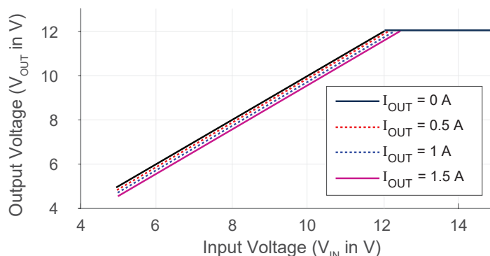
Figure 9: 12 V Output Voltage Dropout at Low V_{IN}
