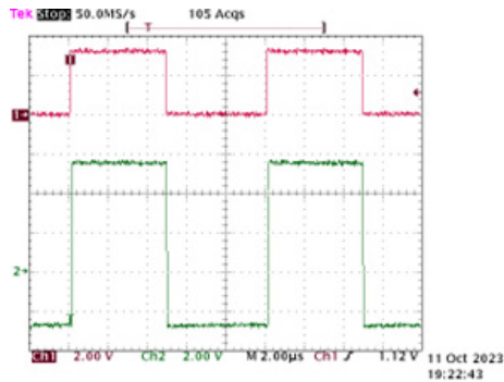
CH1: Driver Input CH2: Driver Output wrt VHV- Low-Side Driver Output
