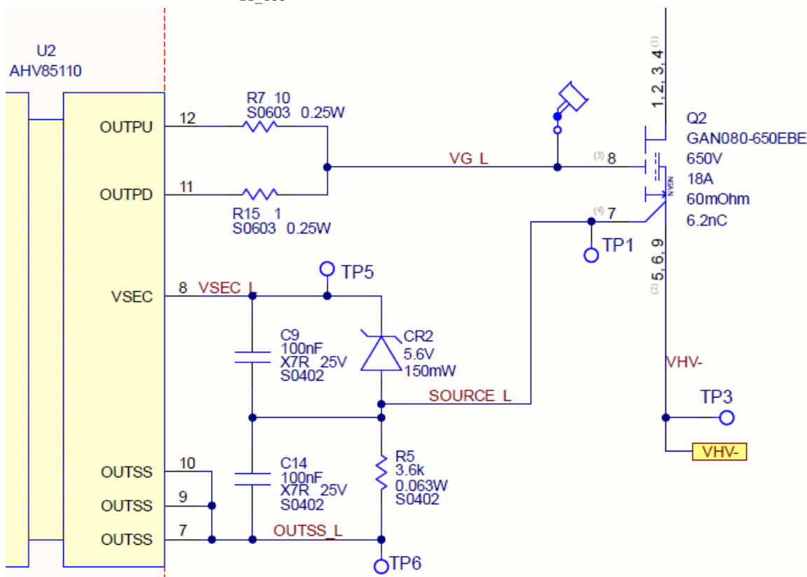
Figure 6: Bipolar Gate-Drive Schematic
