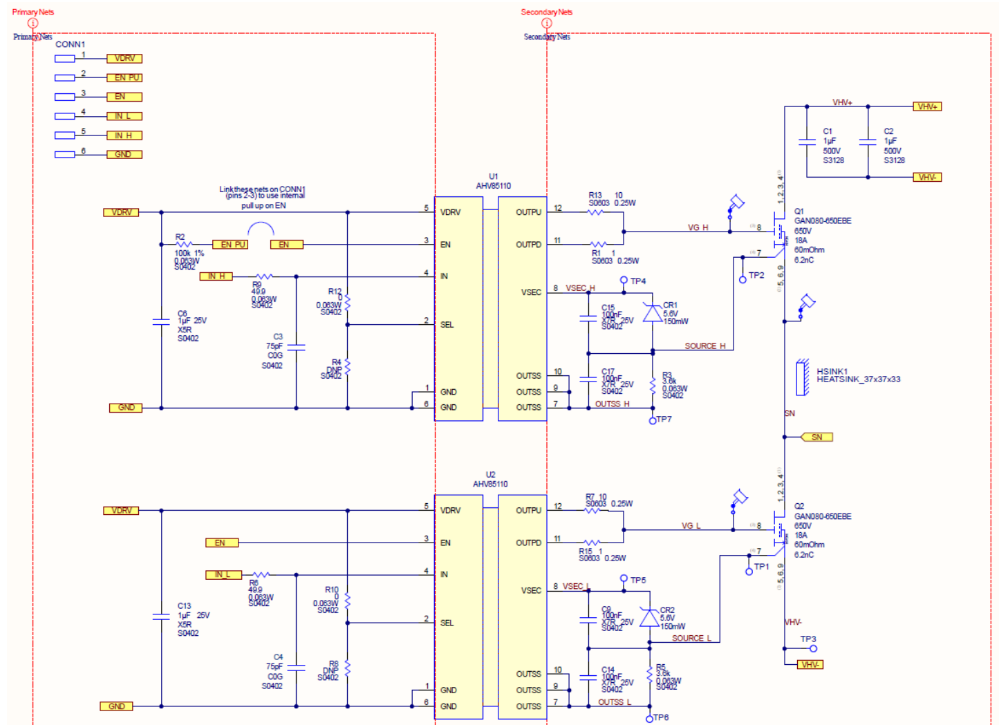
Figure 12: APEK85110KNH-05-T-MH Schematic
