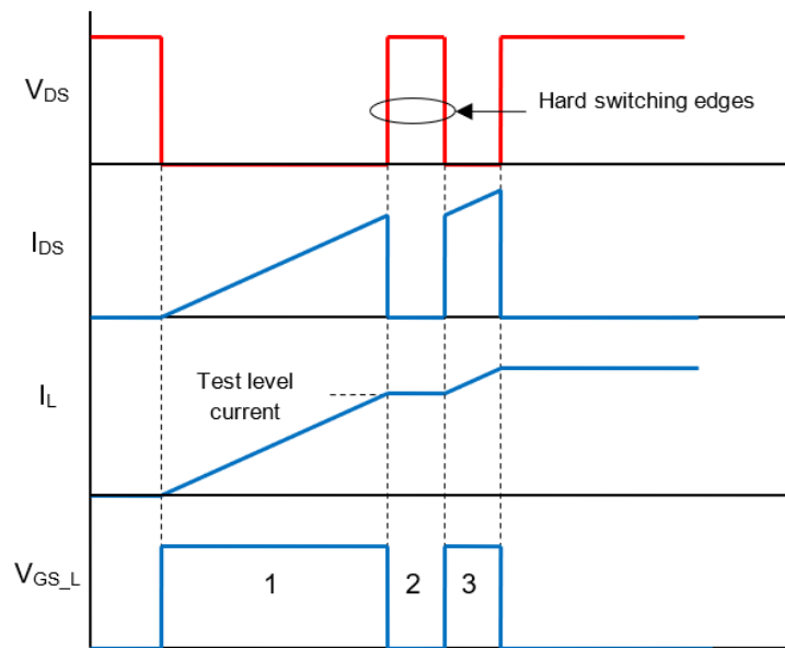
The low-side switch is driven with two pulses as shown in Figure 9. The high-side switch can be held off or driven with the inverse of the low-side gate switch (with adequate dead time).
