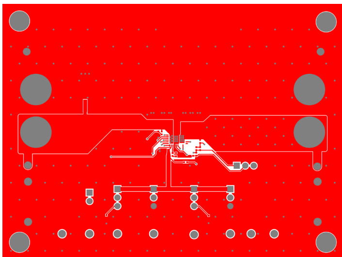
Figure 10: Top Layer
