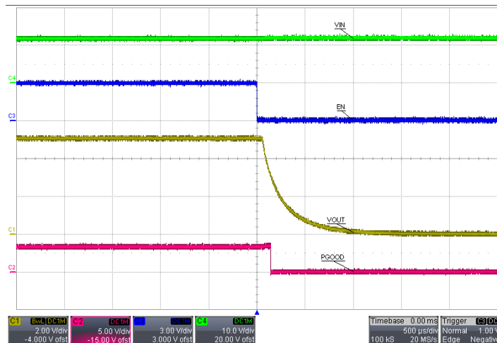
Figure 4: Shutdown with EN Signal; 5 \Omega load applied to VOUT
