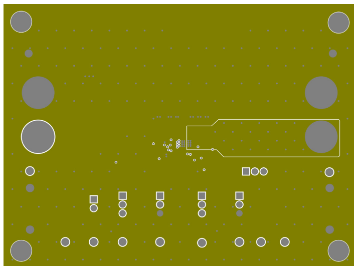
Figure 12: Inner Layer 2 (PGND Plane)
