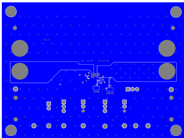
Figure 13: Bottom Layer
