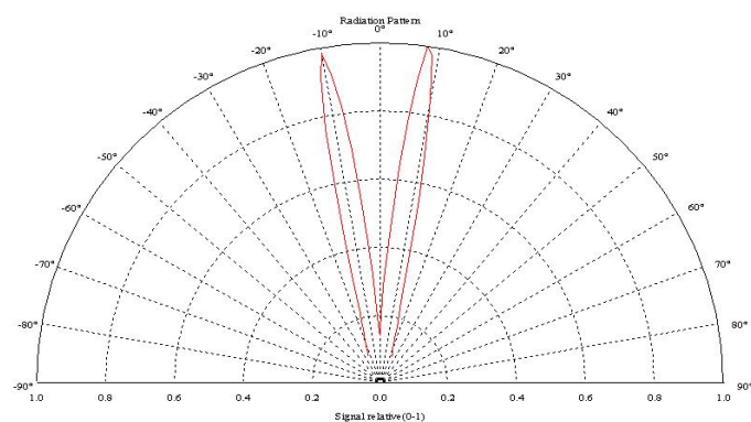
RADIATION PATTERN
