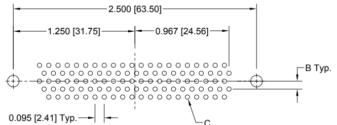
DD104 FEMALE
