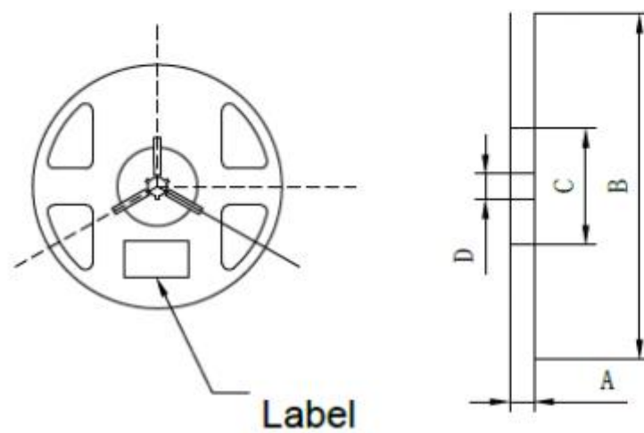
Reel Dimension
