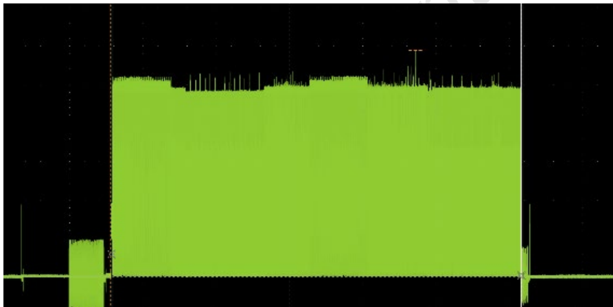
Figure 3-2 Image Update Current Profile
