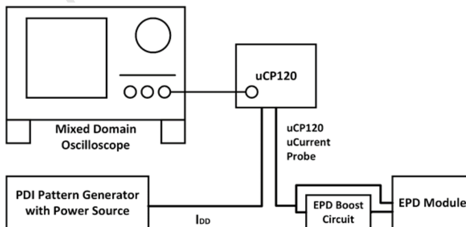
Figure 3-3 Current Measurement
