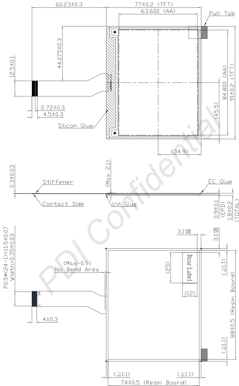
Figure 1-1 EPD Drawing
