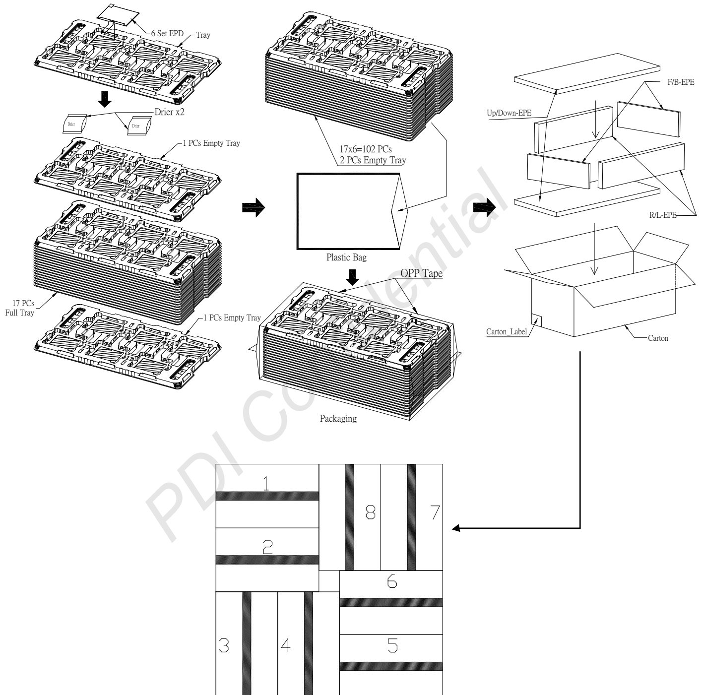
Figure 7-1 Packing Diagram
