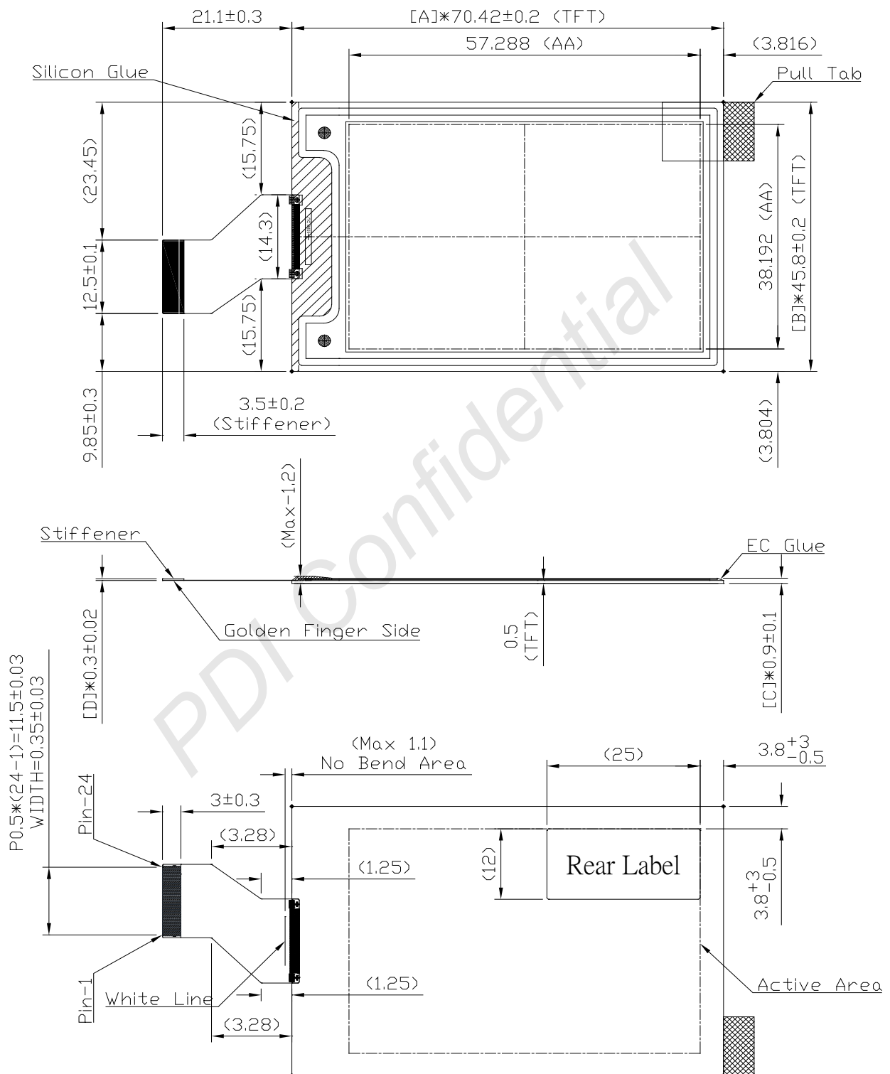
Figure 1-1 EPD Drawing
