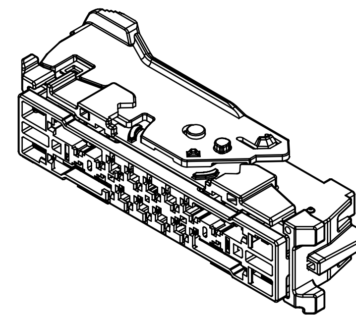
FRONT ISOMETRIC VIEW (SHIPPING POSITION) (1/1)
