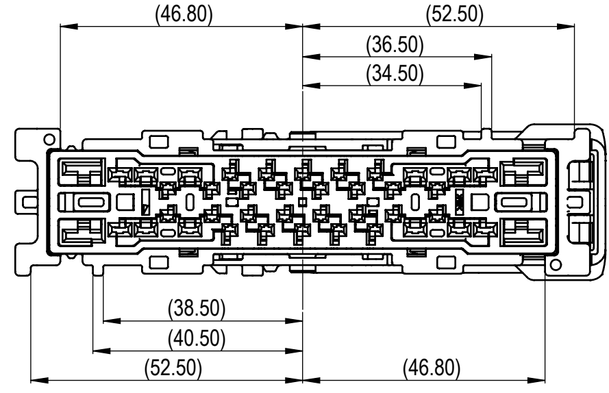
7287-8886-90 KEYWAY D RIGHT
