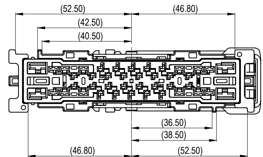
7287-8880-30 KEYWAY A RIGHT
