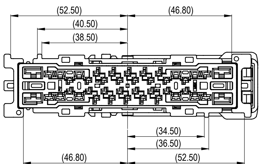
7287-8882-40 KEYWAY B RIGHT
