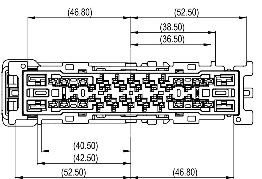
7287-8883-60 KEYWAY C LEFT
