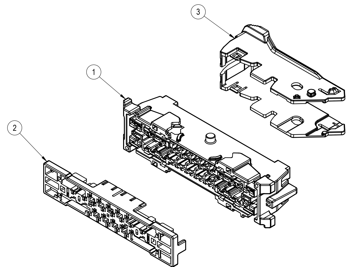
EXPLODED VIEW (1/1)
