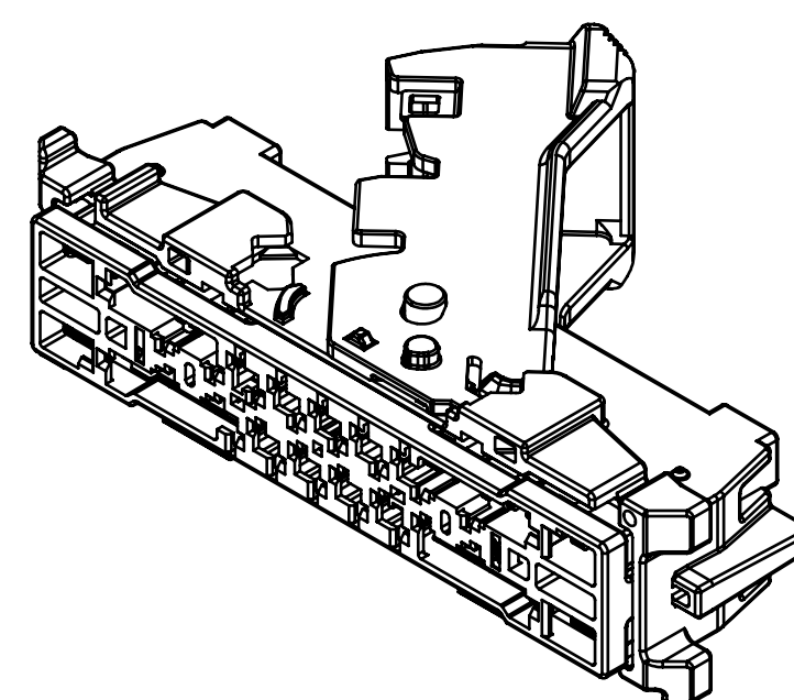
FRONT ISOMETRIC VIEW (LEVER IN PRE-SET POSITION) (1/1)
