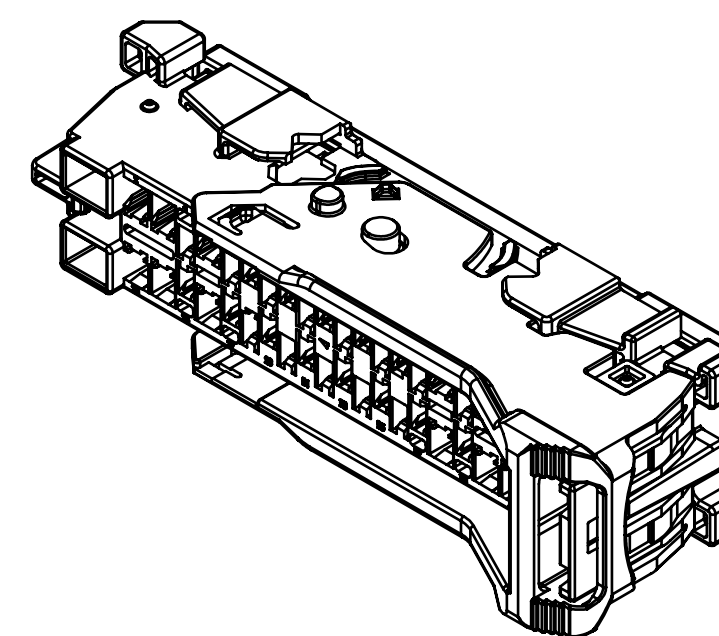
REAR ISOMETRIC VIEW (1/1)
