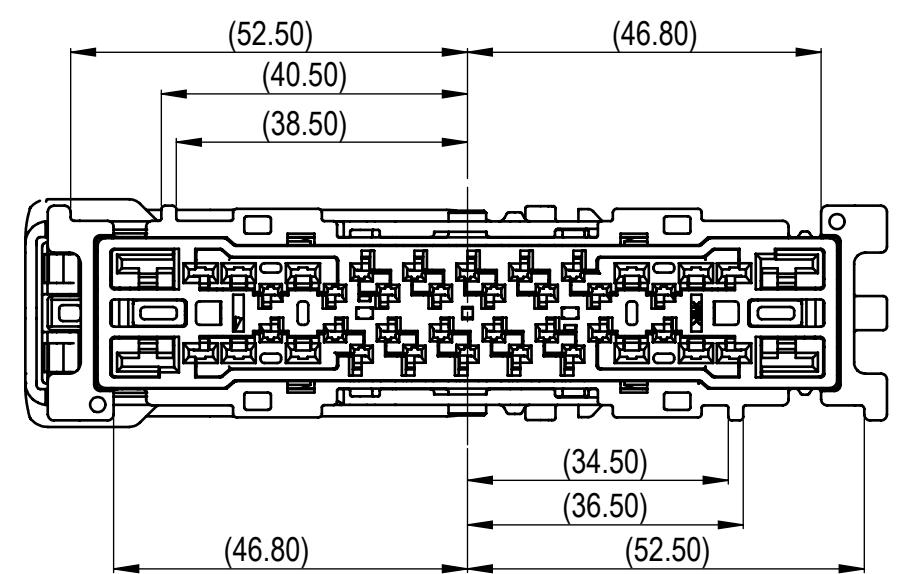
7287-8881-40 KEYWAY B LEFT
