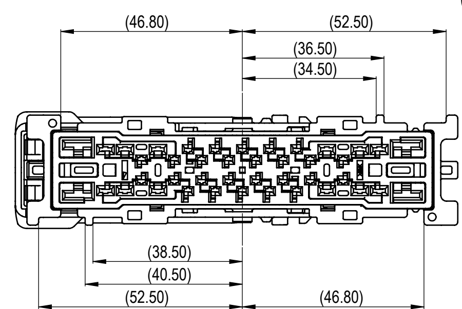
7287-8885-90 KEYWAY D LEFT
