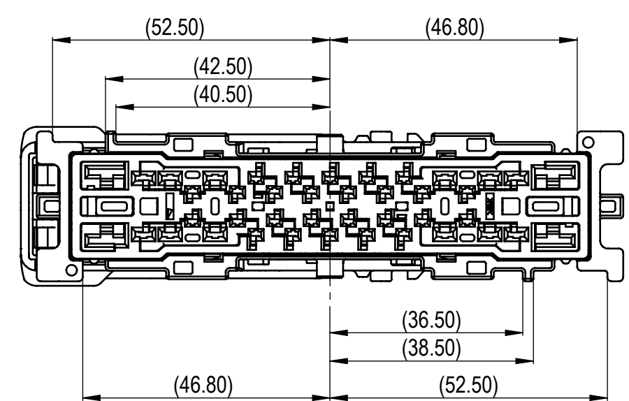
7287-8879-30 KEYWAY A LEFT
