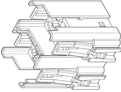
ISOMETRIC VIEW
