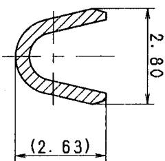
SEC. A-A (10/1)
