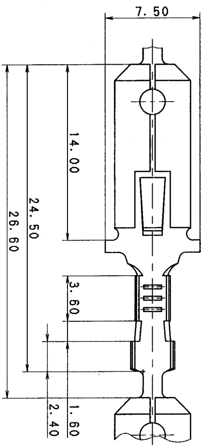
SEC. A-A (10/1)
