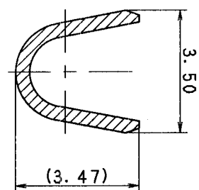
SEC. B-B (10/1)
