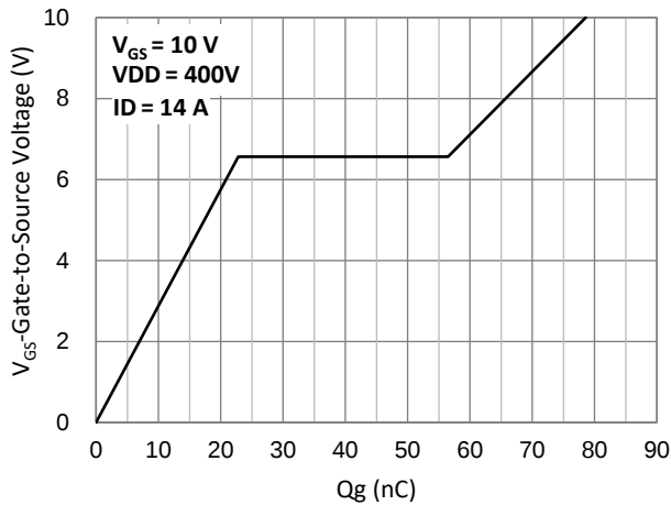
Fig.7 Gate-Charge Characteristics
