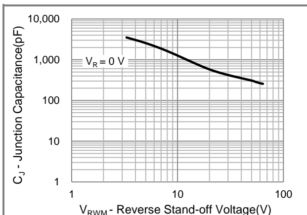
Fig.4 Typical Capacitance
