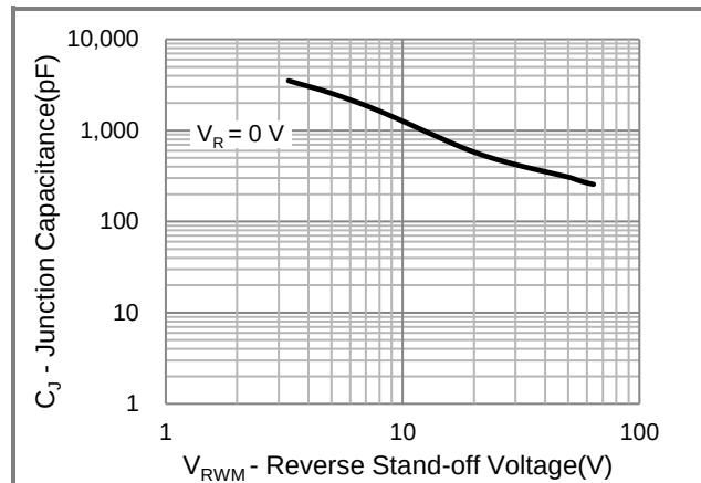
Fig.4 Typical Capacitance
