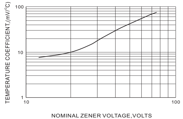
Fig.2 TEMPERATURE COEFFICIENTS
