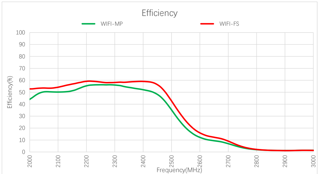
Efficiency (%) - Wi-Fi
