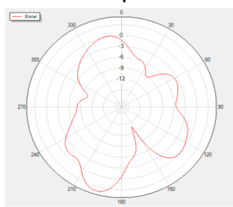
Phi=90 Freq=1880MHz
