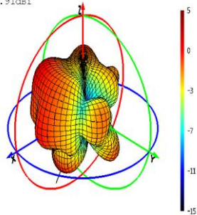
Phi=0 Freq=1880MHz
