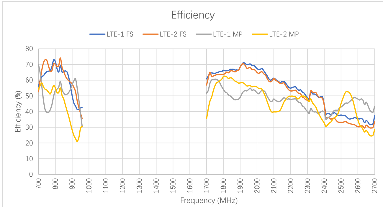
Efficiency (%) - LTE
