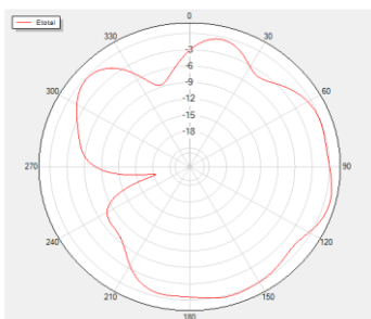
Phi=0 Freq=2140MHz
