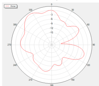
Theta=90 Freq=2140MHz
