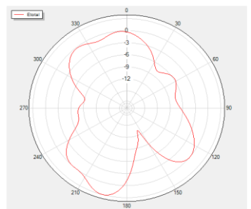
Phi=90 Freq=1950MHz
