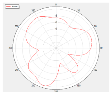
Phi=90 Freq=2350MHz
