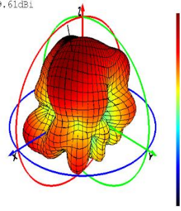
Phi=0 Freq=2350MHz
