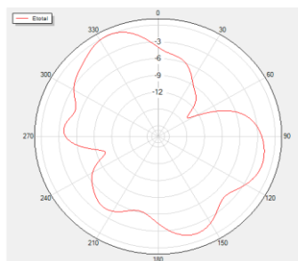
Phi=0 Freq=2350MHz
