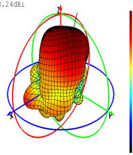
Phi=0 Freq=2600MHz
