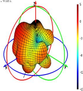
Phi=0 Freq=1950MHz
