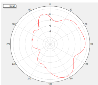
Phi=0 Freq=1880MHz
