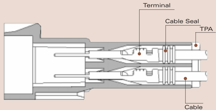
Male Connector
