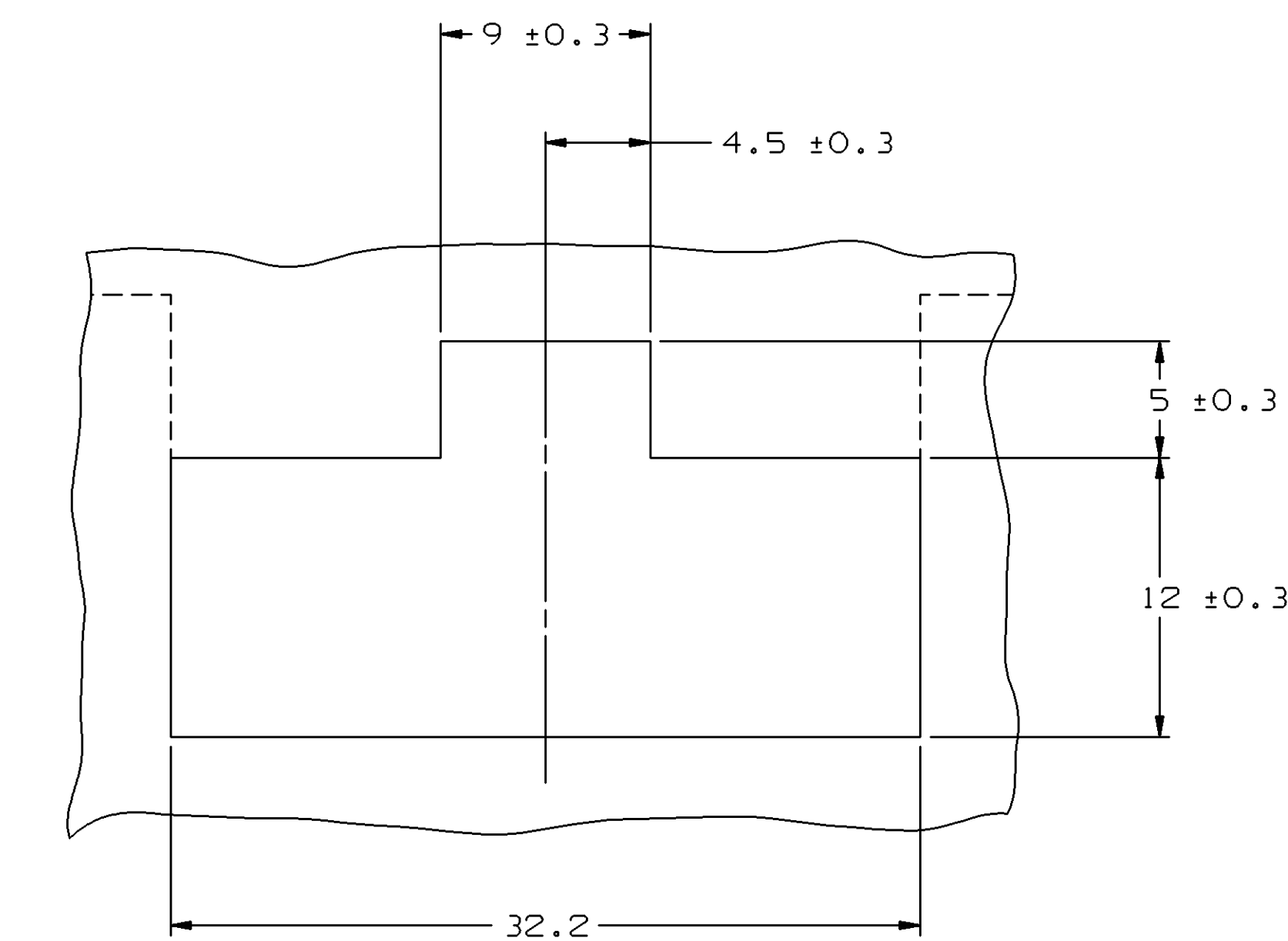
MOUNTING HOLE (VIEWED FROM OUTSIDE OF CASE)
