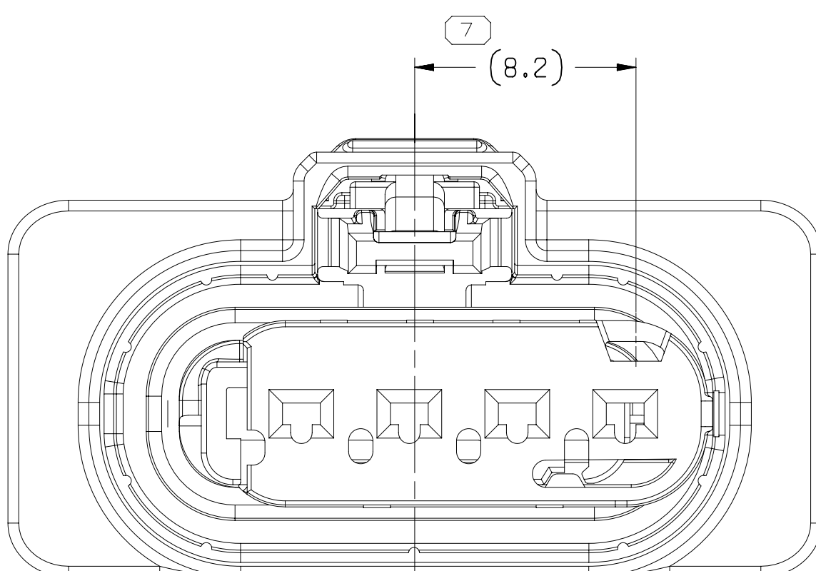
TYPE 208 SAME AS TYPE 20 EXCEPT AS SHOWN
