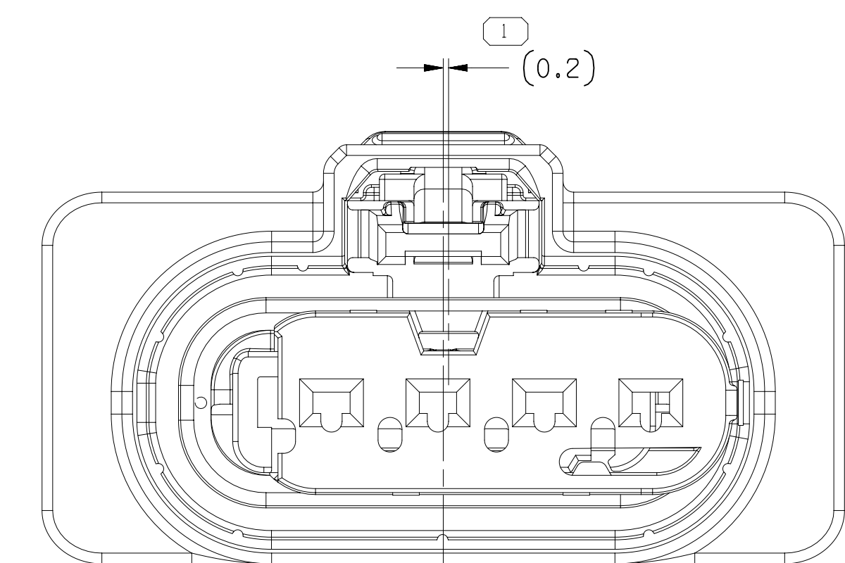
TYPE 202 SAME AS TYPE 200 EXCEPT AS SHOWN
