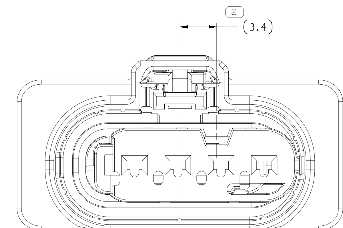
TYPE 203 SAME AS TYPE 20 EXCEPT AS SHOWN
