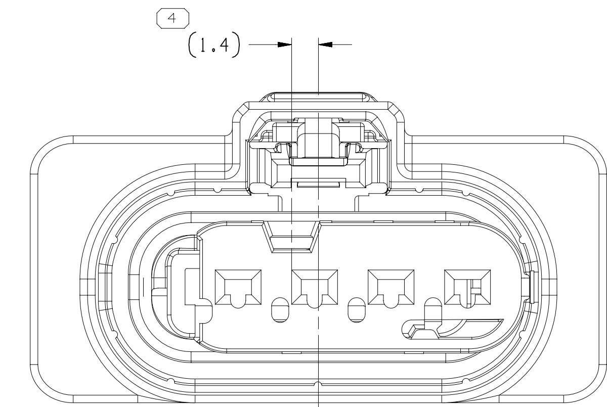
TYPE 205 SAME AS TYPE 20 EXCEPT AS SHOWN
