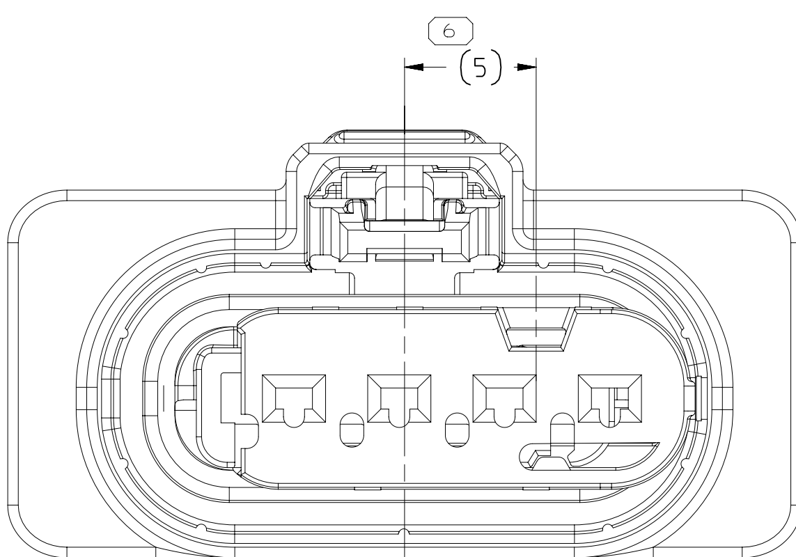
TYPE 207 SAME AS TYPE 201 EXCEPT AS SHOWN
