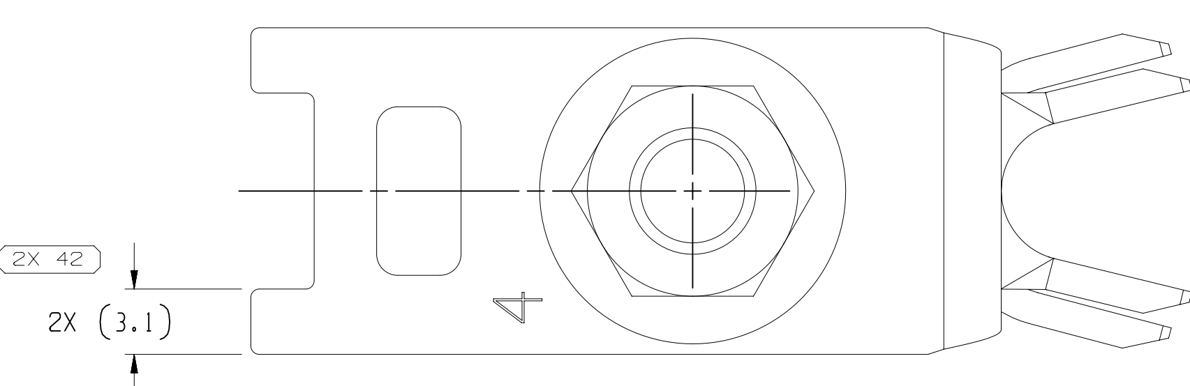
TYPE 216 12-19 MM 2 SAME AS TYPE 205 EXCEPT AS SHOWN
