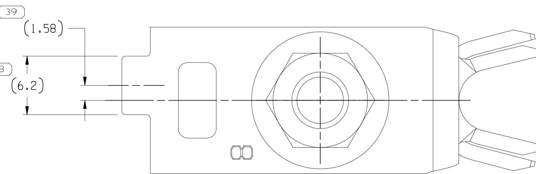
TYPE 214 20-35 MM 2 SAME AS TYPE 205 EXCEPT AS SHOWN
