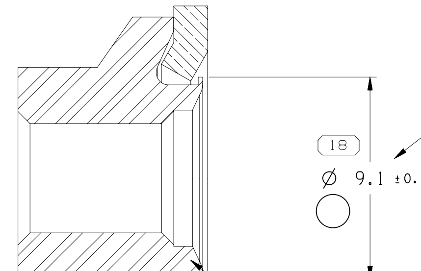
SECTION A-A SCALE 6:1
