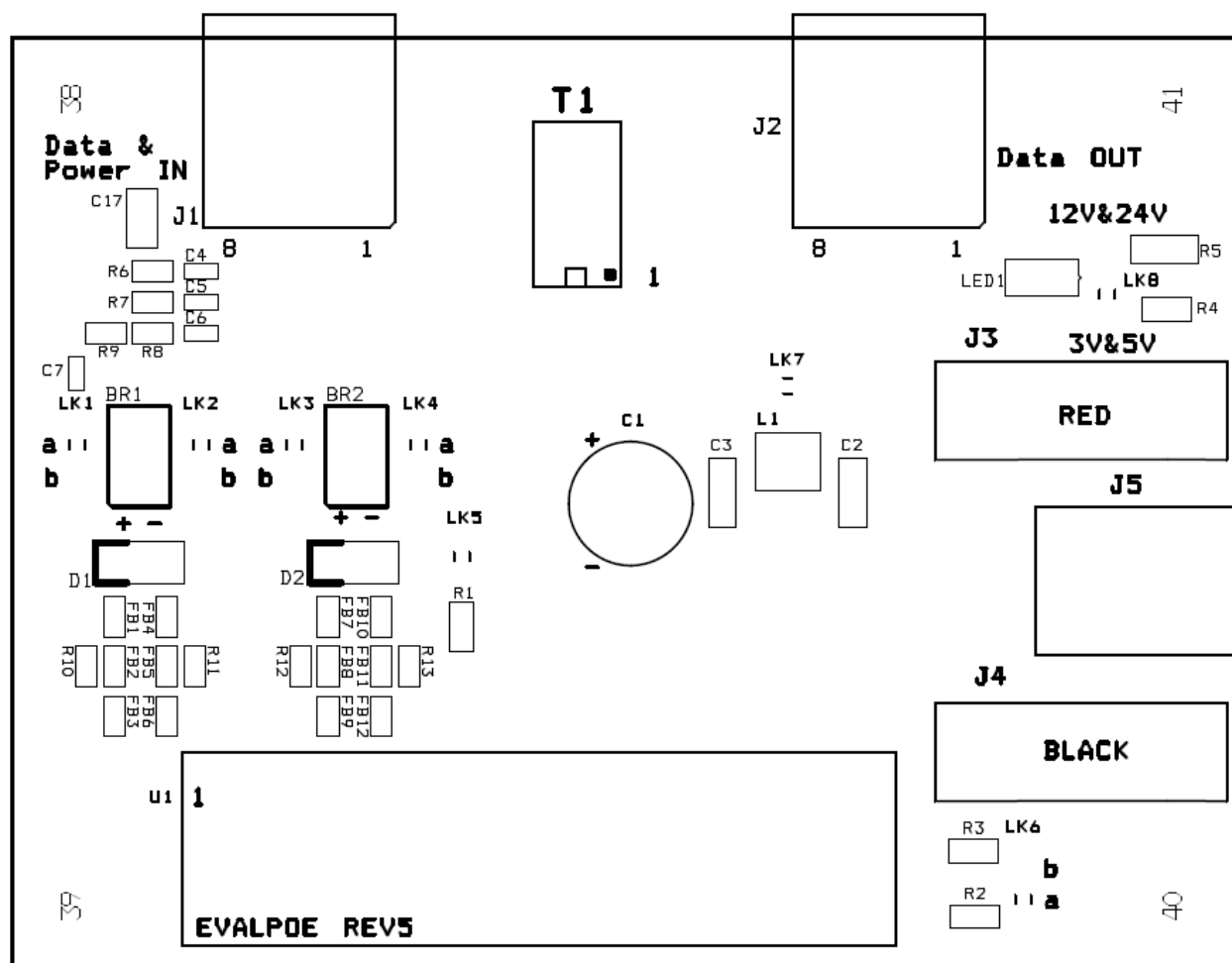
Figure 1: Board Layout
