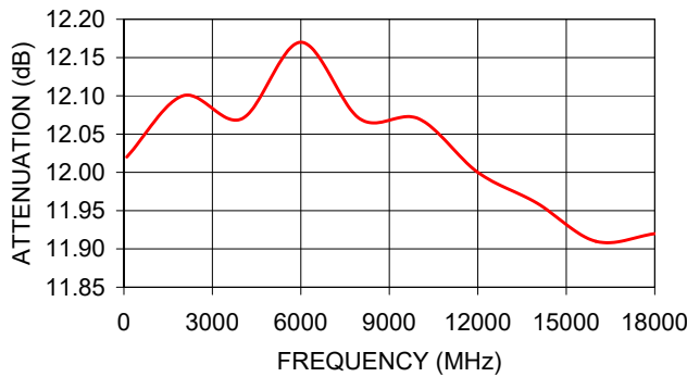
BW-S12W5+ ATTENUATION
