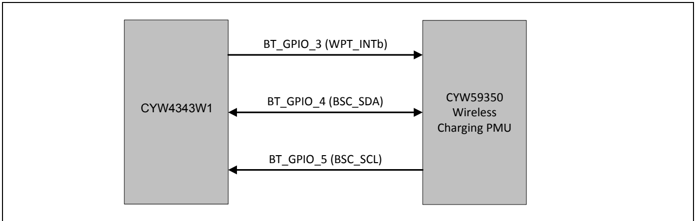
Figure 8. CYW4343W1 Interface to a CYW59350
