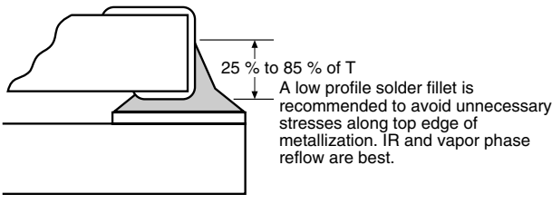
FIGURE 4 - RECOMMENDED MOUNTING 1)2)3)
