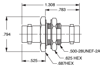
FEED-THROUGH JACK TWO-PIN POLARIZED
