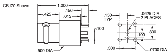
TWINAX/TRIAX TRB CONCENTRIC CIRCUIT BOARD JACK
