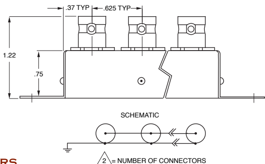
ADAPTERS MULTIPLE PARALLEL NETWORK 50Ω MPN-△/BNC 50Ω MPN-△/TNC Contact the factory for more information.
