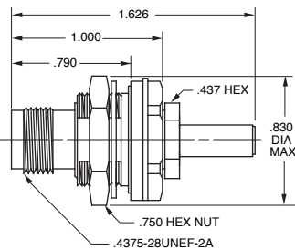
INSULATED BULKHEAD JACK REAR MOUNT, TOOL CRIMP 50Ω BJ246-001 75Ω UBJ246-001 Mounting Hole: D2.187 GF-Ground filter version pg 43
