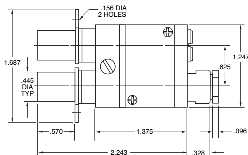
PATCH JACK SINGLE ENTRY WITH 20 dB ISOLATED MONITORING JACK ENTRY TRB 3-LUG TRT THREADED CABLE (SHOWN)
