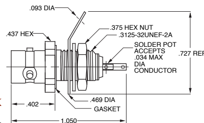
HERMETICALLY SEALED BULKHEAD JACK 3-lug BJ157HS 4-lug BJ157FLHS Mounting Hole: D6.187
