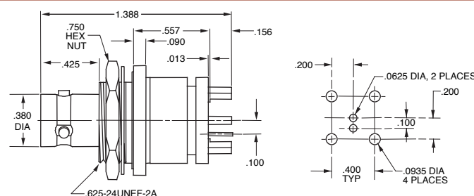
TWINAX/TRIAX TRB INSULATED CONCENTRIC FEMALE 3-LUG BULKHEAD MOUNT
