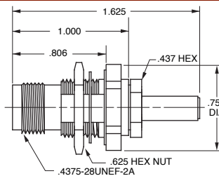
BULKHEAD CABLE JACK WRENCH CRIMP 50Ω BJ49-1 75Ω UBJ49-1 Mounting Hole: D3.218 / D2.218 (Cable Groups 6, 6E, 51, 52)
