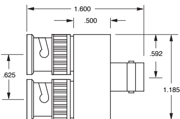
ADAPTER FIXED PARALLELING 50Ω BNC-Two jacks, One plug PN2C
