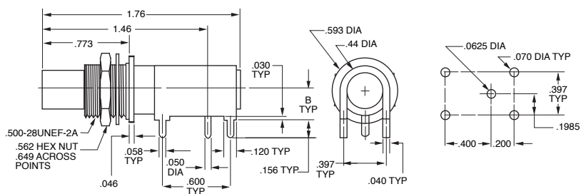
CIRCUIT BOARD BULKHEAD MOUNTING MINI-WECO PATCH JACK
