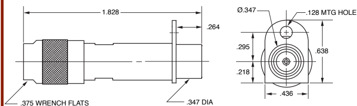
MINIATURE PATCH JACK CABLE ENTRY, FIELD SERVICEABLE MINI-WECO TYPE Minimum .64" centers
