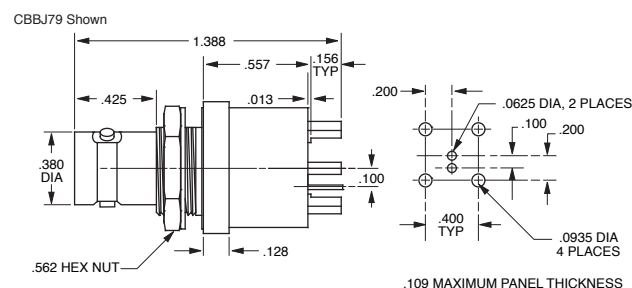
TWINAX/TRIAX TRB NON-INSULATED CONCENTRIC FEMALE 3-LUG BULKHEAD MOUNT
