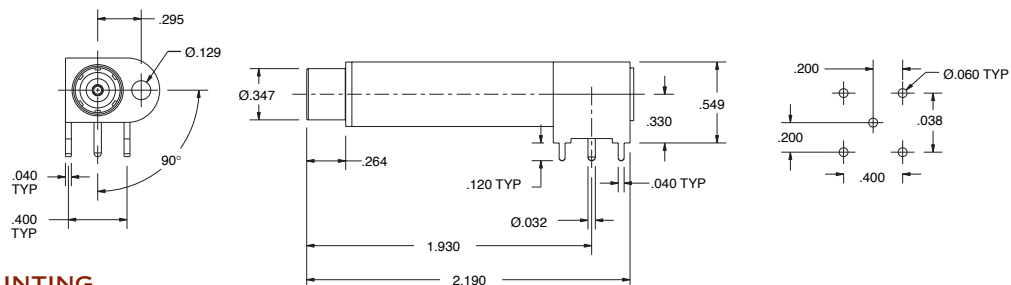
CIRCUIT BOARD MOUNTING MINI-WECO COAXIAL PATCH JACK RIGHT ANGLE 75 \Omega (.296 SIZE)
