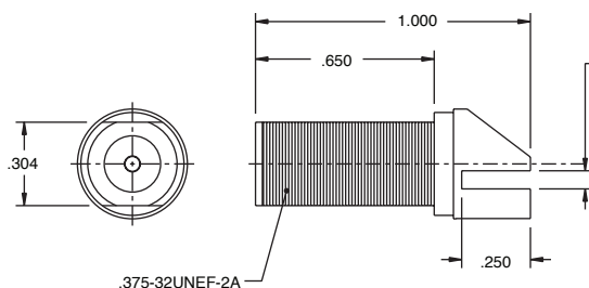
CIRCUIT BOARD EDGE MOUNT "F" STYLE FEMALE JACK CBJE130-1, -2, or -3
