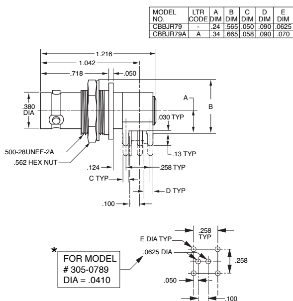
RIGHT ANGLE CIRCUIT BOARD BULKHEAD JACK
