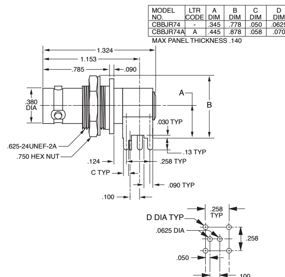
RIGHT ANGLE INSULATED CIRCUIT BOARD BULKHEAD JACK
