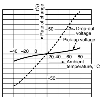
5.-(1) Change of pick-up and drop-out voltage (1a type) Sample: DSP1a-DC12V, 5 pcs.
