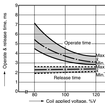
4.-(4) Operate & release time (with diode, 1a type) Sample: DSP1a-DC12V, 5 pcs.
