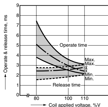
4.-(5) Operate & release time (with diode, 1a1b type) Sample: DSP1-DC12V, 5 pcs.
