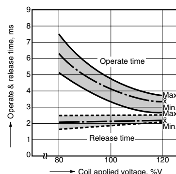
4.-(6) Operate & release time (with diode, 2a type) Sample: DSP2a-DC12V, 5 pcs.
