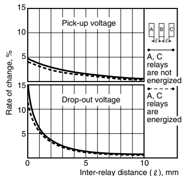
6.-(1) Influence of adjacent mounting (1a type) Sample: DSP1a-DC12V, 5 pcs.
