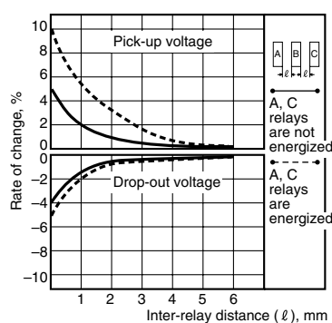
6.-(2) Influence of adjacent mounting (1a1b type) Sample: DSP1-DC12V, 5 pcs.
