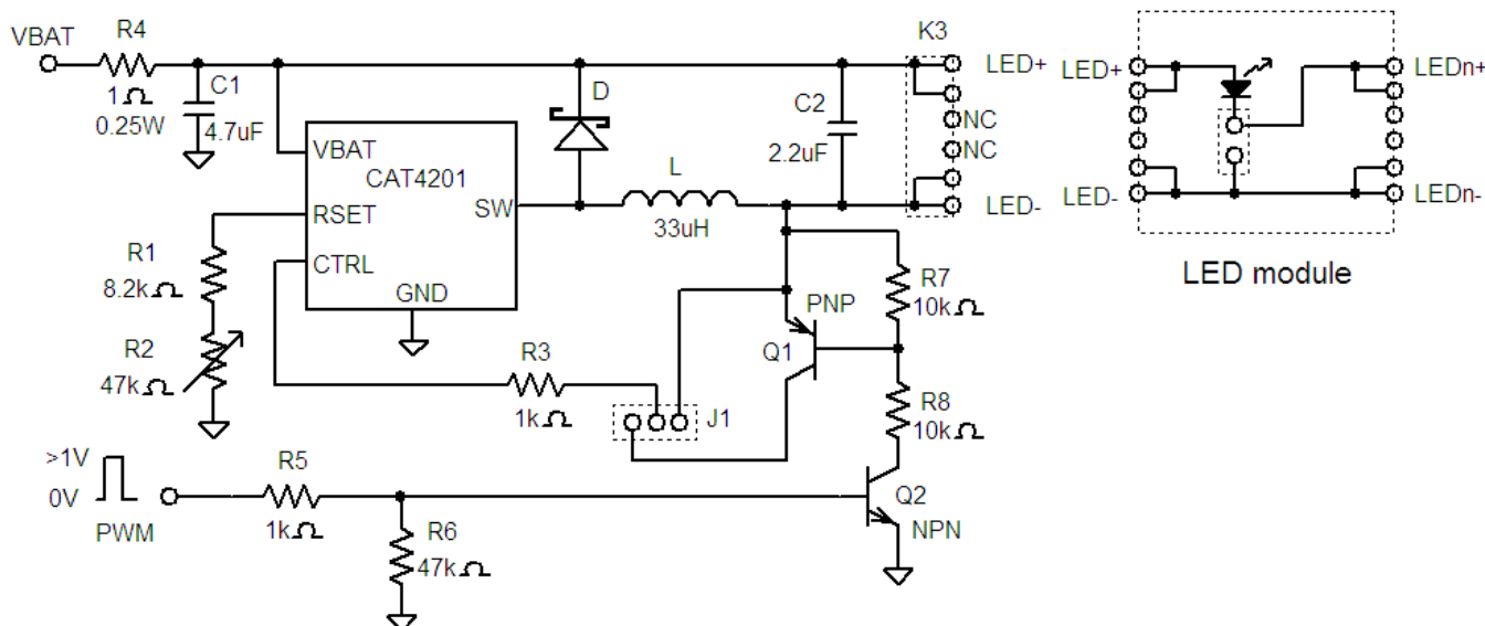
Figure 2. CAT4201EVAL2 Schematic
