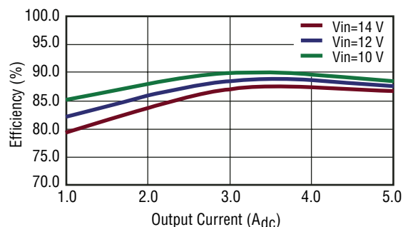
Fig. 4 Efficiency vs. Output Current ( V_{out} = 2.5 V_{dc} )
