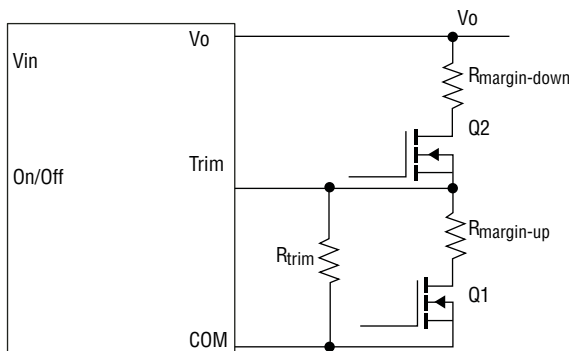
Fig. 25 Circuit Configuration for Margining Output Voltage
