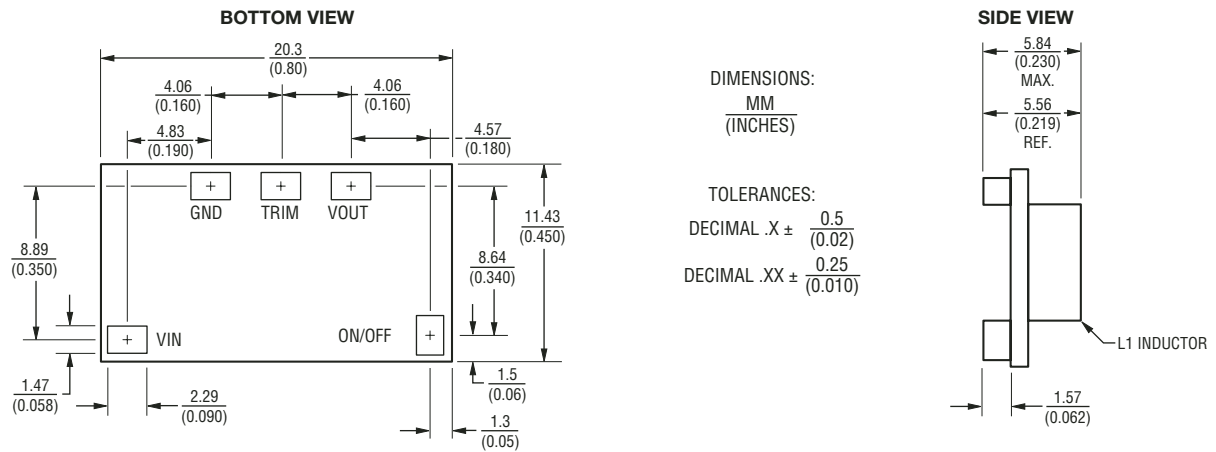
Fig. 28 Product Dimensions
