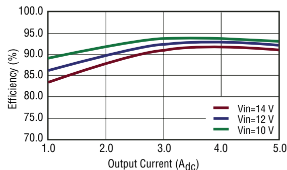
Fig. 6 Efficiency vs. Output Current ( V_{out} = 5.0 V_{dc} )
