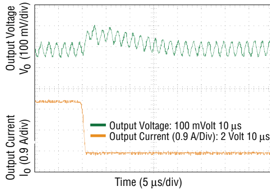
Fig. 13 Transient Response - 5 A - 2.5 A Step ( V_{in} = 12 V_{dc} , V_O = 3.3 V_{dc} , C_{ext} = 2 \times 100 \mu F Polymer Caps)
