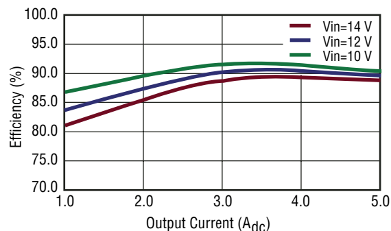
Fig. 5 Efficiency vs. Output Current ( V_{out} = 3.3 V_{dc} )
