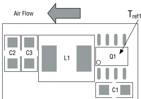
Fig. 26 T_{ref1} Temperature Measurement Location
