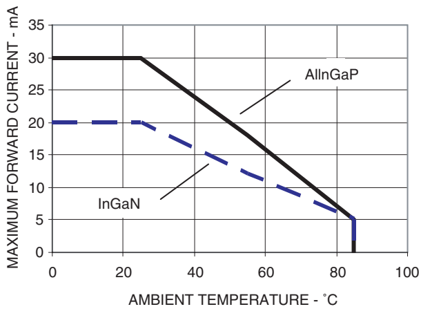
Figure 7. Maximum forward current vs. ambient temperature
