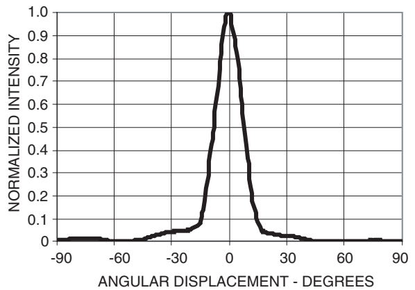
Figure 8. Radiation Pattern For AllnGaP & InGaN Derating based on T_{JMAX} = 95^\circ
