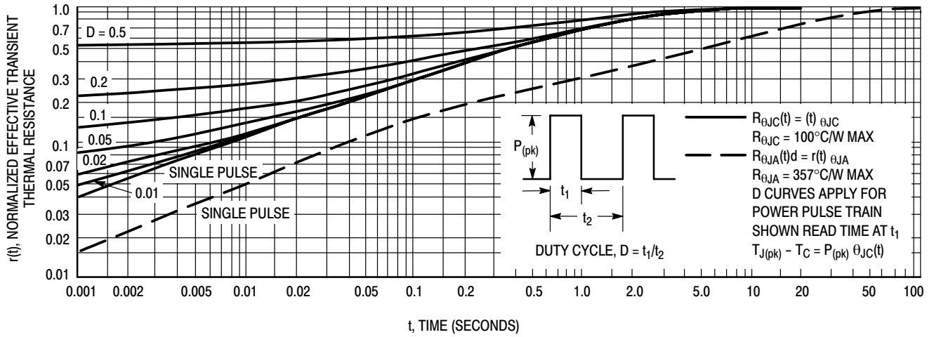
Figure 1. Thermal Response
