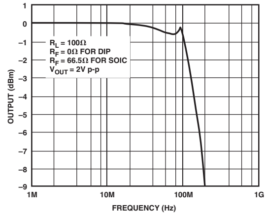
TPC 16. AD8047 Large Signal Frequency Response, G = +1
